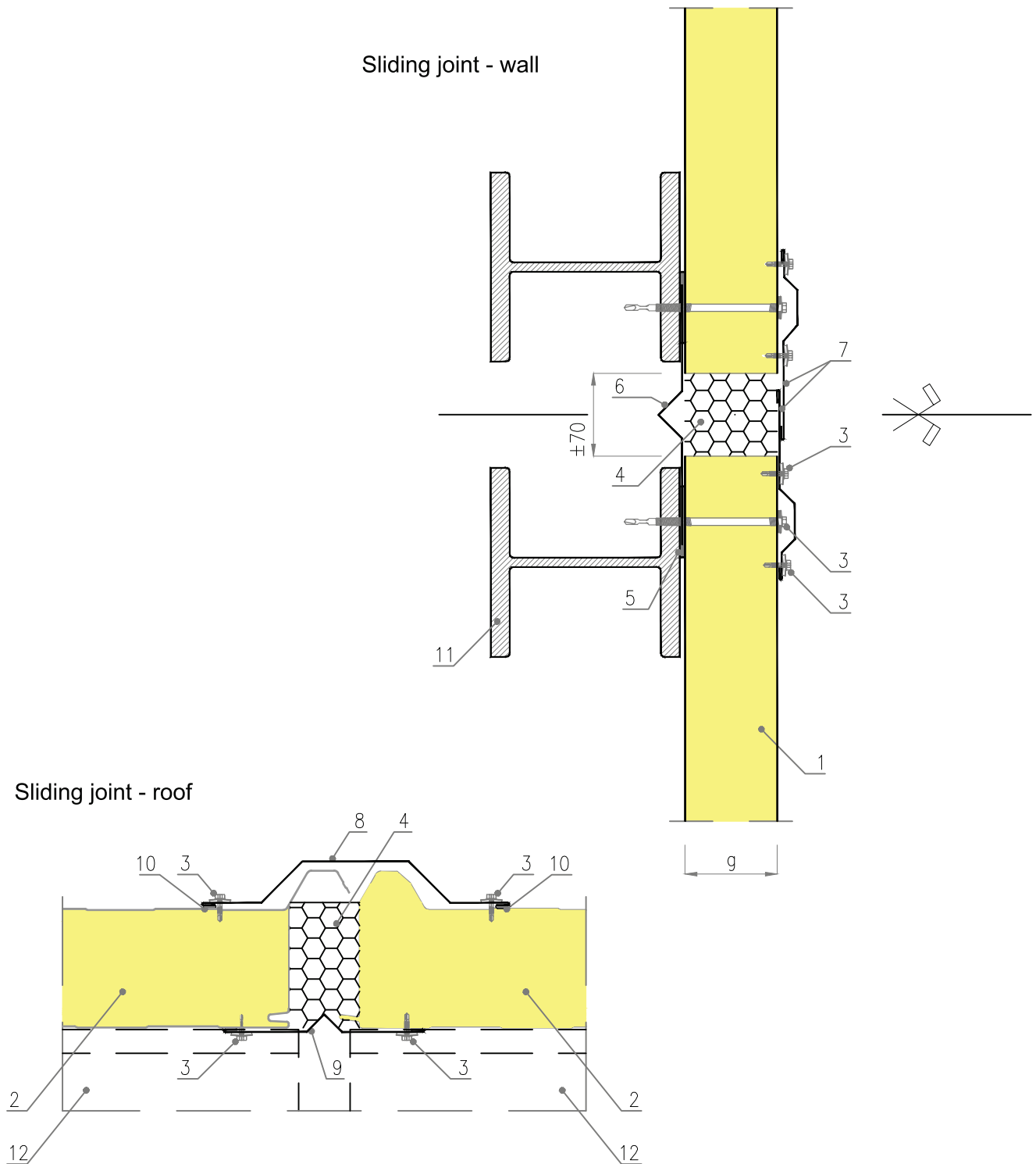
Drawing 16. S Panel Wall, S Panel Roof PIR; MWF; EPS - sliding joint
