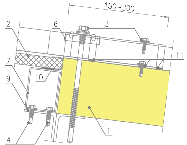
Joint on the longer side of the roof panel with skylight on the side of the eaves
