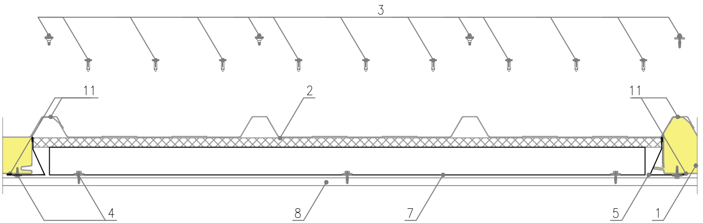
Joint on the longer side of the roof panel with skylight on the side of the roof ridge
