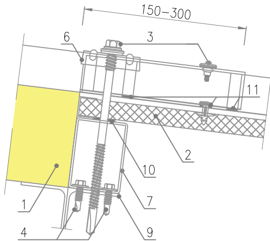
Joint on the longer side of the roof panel with skylight on the side of the roof ridge
